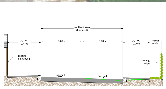
TYPICAL CROSS SECTION K-K SCALE 1:50
