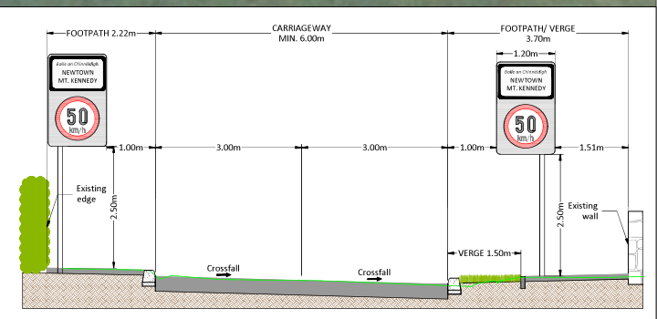
TYPICAL CROSS SECTION L-L SCALE 1:50
